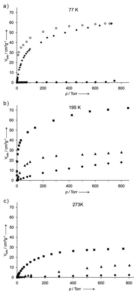
Figure 2. H 2 (◆), N 2 (●), CO 2 (■), and CH 4 (▲) adsorption isotherms for 1 at a) 77, b) 195, and c) 273 K; open symbols denote desorption.
